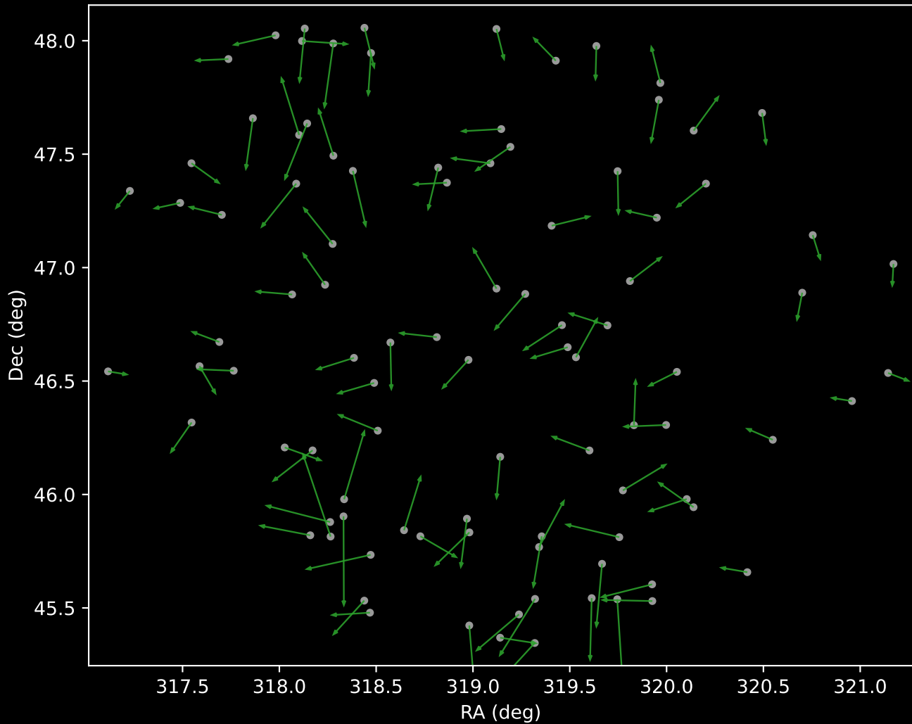
APOGEE DR17 Cluster 4 Proper Motion Vectors (n=96)
