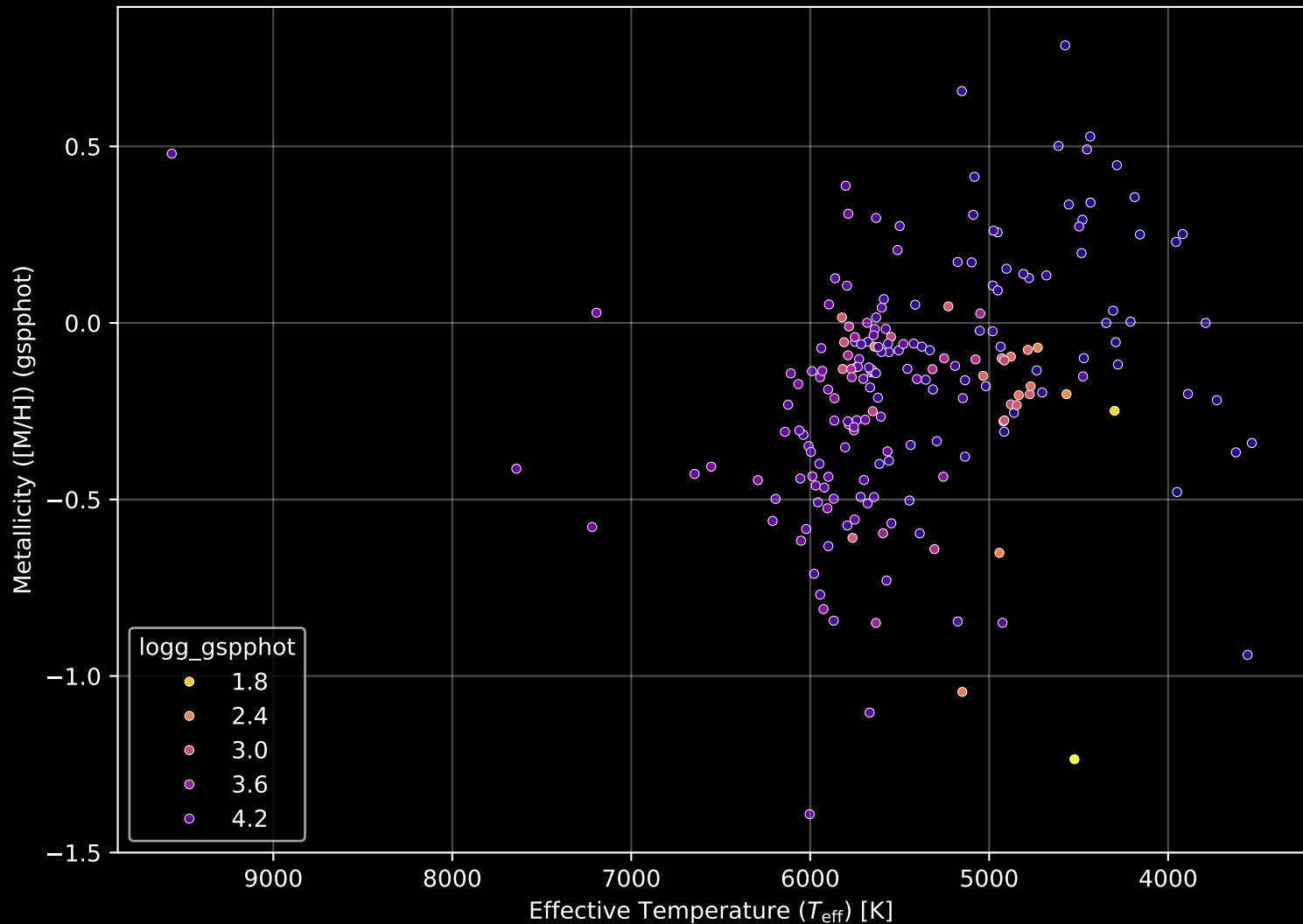
APOGEE DR17 Field: [084+62_MGA] Stellar Population Parameters (n= 202)
