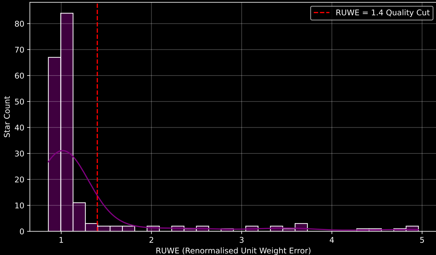
GAPOGEE DR17 Field [084+62_MGA] RUWE Distribution (n= 192)
