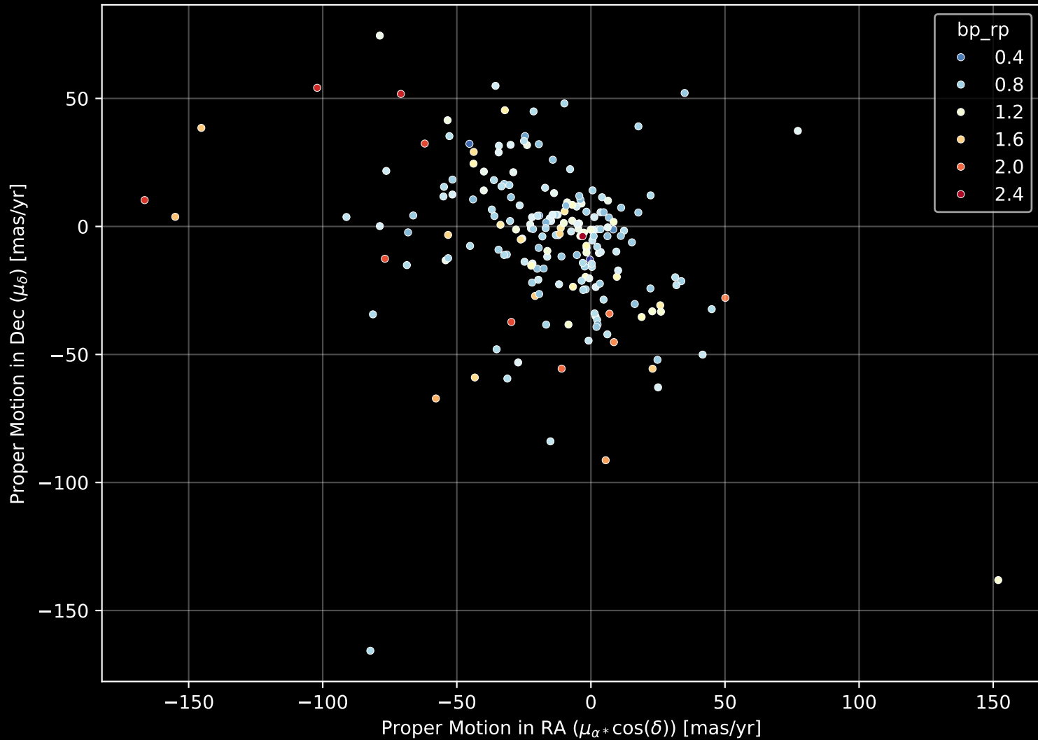
APOGEE DR17 Field: [084+62_MGA] Proper Motion Diagram (n= 202)
