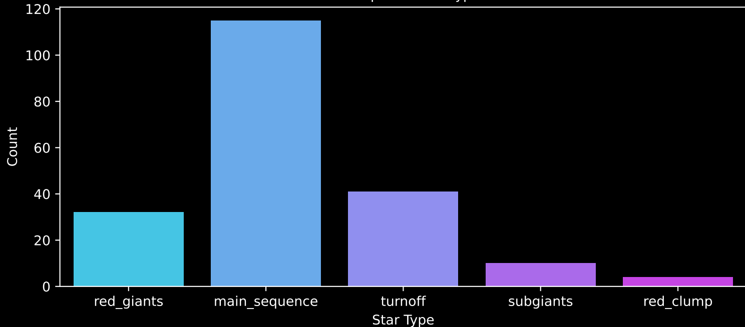
APOGEE DR17 Field: [084+62_MGA] Count plot of Star Type
