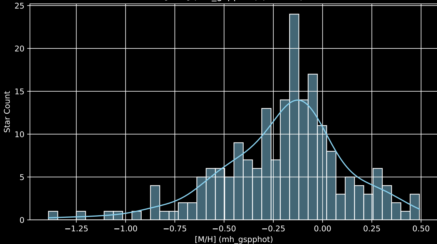
APOGEE DR17 Field: [084+62_MGA [M/H] (mh_gspphot) (n= 198)
