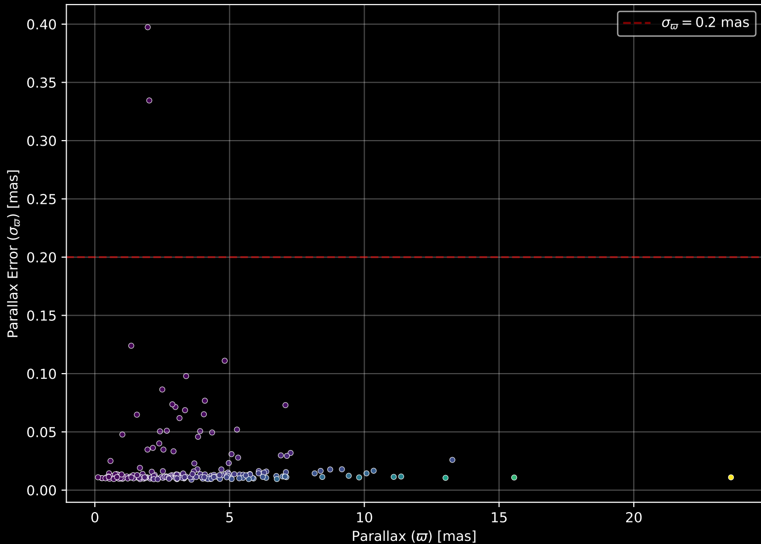
APOGEE DR17 Field: [084+62_MGA] Parallax Quality (n= 202)
